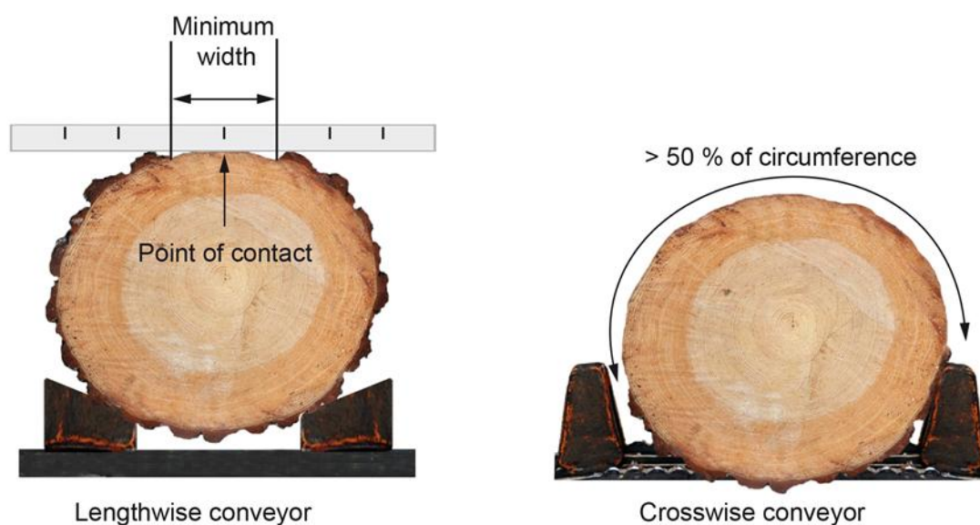
Figure 7. Principles for assessing bark abrasion when measuring logs on lengthwise conveyors (left) and crosswise conveyors (right).
