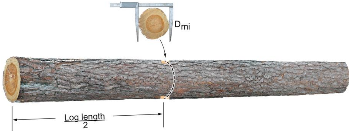
Figure 11. Measurement point for diameter in mid-point measurement.
