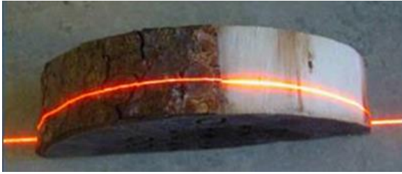
Figure 8. Principle of diameter measurement under bark using the tracheid method The laser beam used in the scanner is more dispersed on wood than on bark. Image analysis measures the width and intensity of the laser beam, distinguishing between wood and bark.
